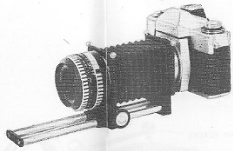
2 Bellows Unit with camera mounted forward
