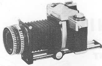
3 Bellows Unit with camera mounted reversed
