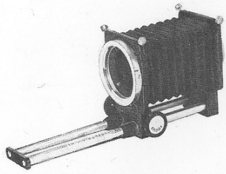
1 B.P.M. Bellows Unit complete with mounts
