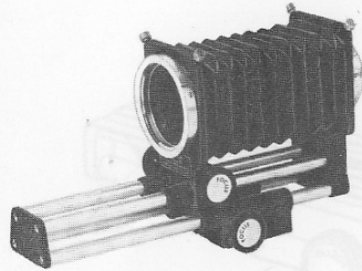
4 NEW B.P.M. BELLOWSIDE with underslide permanently fixed for utmost rigidity
