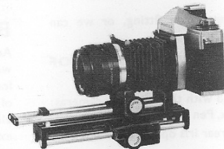
8 B.P.M. BELLOWS mounted on B.P.M. FOCUSLIDE
